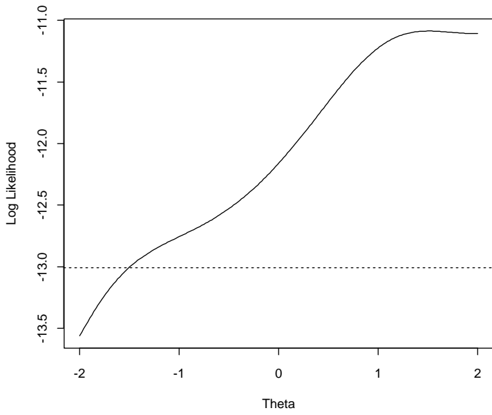
Likelihood Ratio Intervals: Cauchy, n=5
