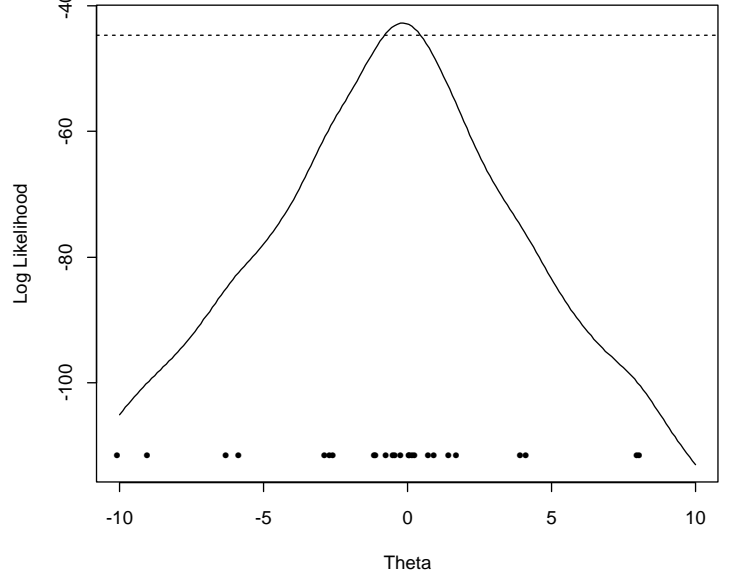
Likelihood Ratio Intervals: Cauchy, n=25
