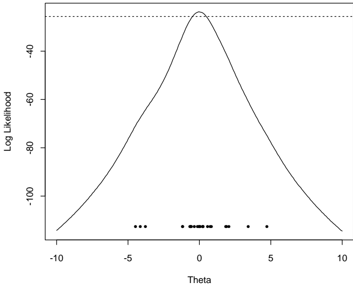
Likelihood Ratio Intervals: Cauchy, n=25
