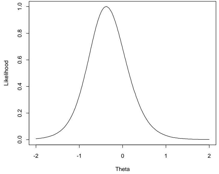
Likelihood Function: Cauchy, n=5
