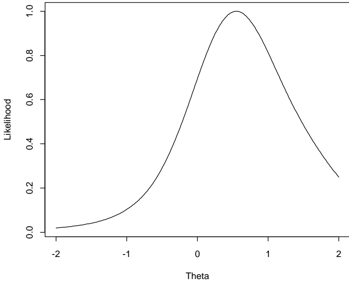
Likelihood Function: Cauchy, n=5
