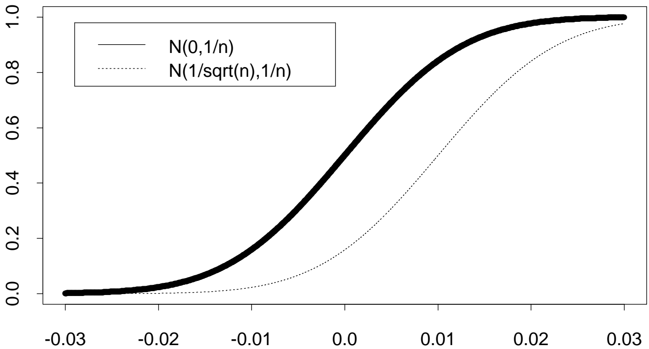
N(1/\sqrt{n}, 1/n) vs N(0, 1/n) ; n=10000
