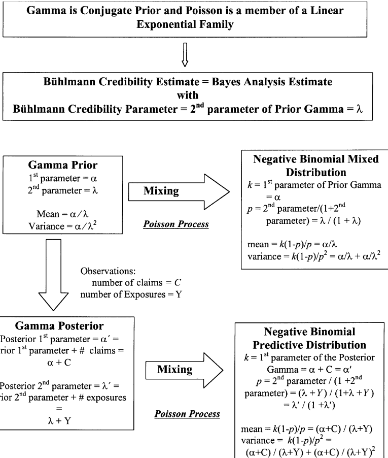
FIGURE 8.4 GAMMA-POISSON FREQUENCY PROCESS
