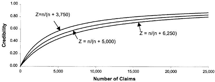
GRAPH 8.6 DIFFERENCE IN K PARAMETER
