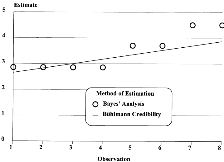
GRAPH 8.3 MULTI-SIDED DIE EXAMPLE
