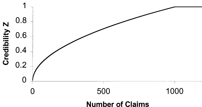
GRAPH 8.1 CLASSICAL CREDIBILITY
