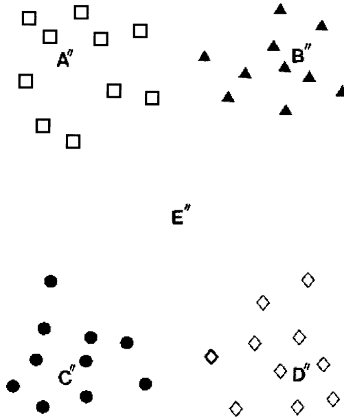
FIGURE 8.3
