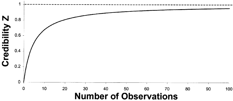
GRAPH 8.2 BÜHLMANN CREDIBILITY
