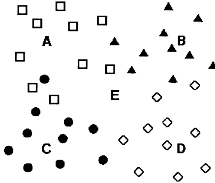
FIGURE 8.1
