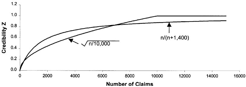
GRAPH 8.7 CLASSICAL VS. BÜHLMANN CREDIBILITY
